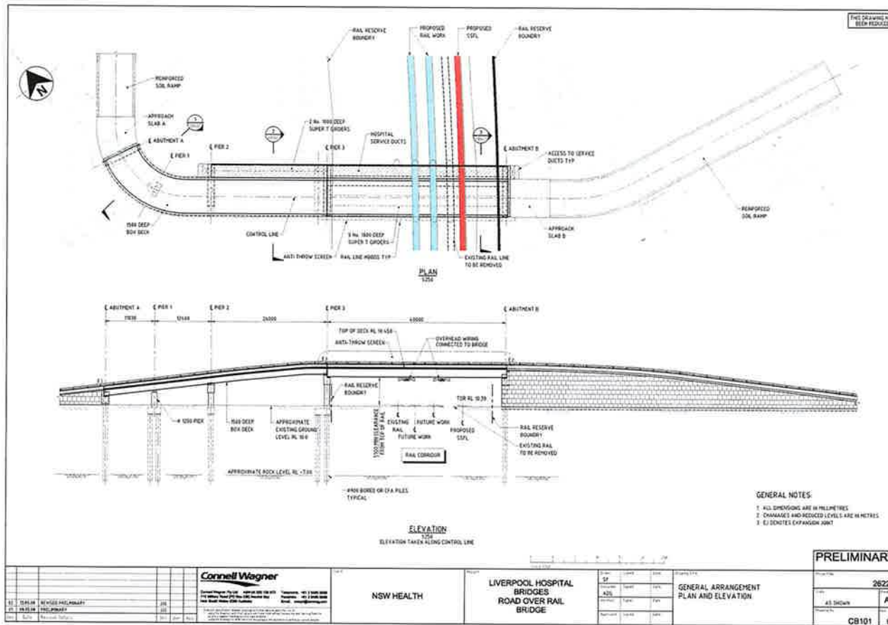
Fig 5.02 - Road Bridge and Approach Ramps
