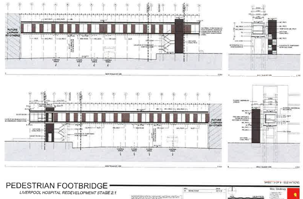
Fig 5.04 - Pedestrian Bridge Elevations
