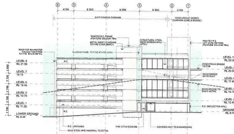
Fig 5.07 - Multi Storey Car Park North Elevation
