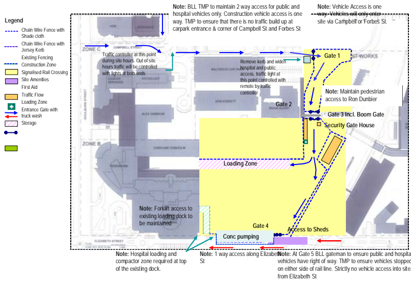
Traffic Management Plan Fencing and Vehicle Movement Stage 2 Nov 08 - Oct 10
