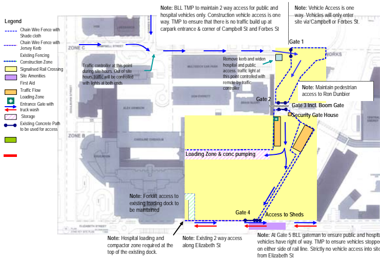
Traffic Management Plan Fencing and Vehicle Movement Stage 1 June 08 - Nov 08
