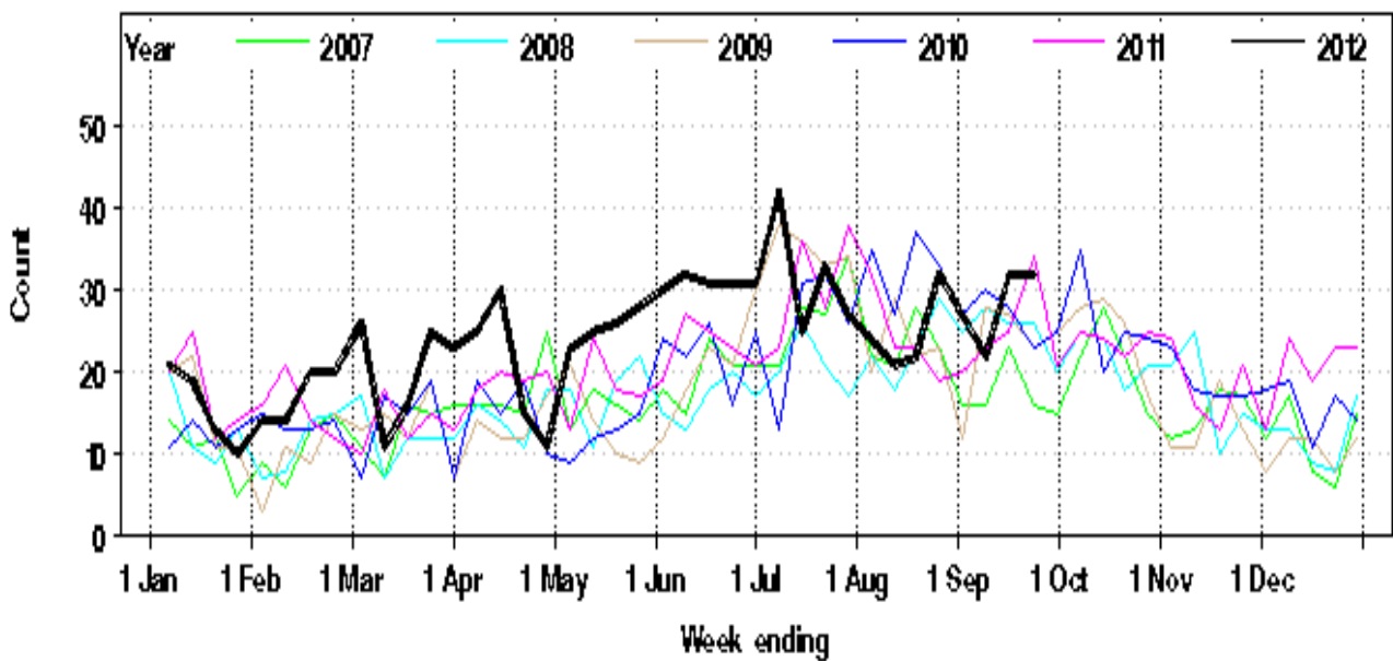
Figure 2: Total weekly counts of Emergency Department visits for pneumonia and influenza-like illness, which were subsequently admitted to a critical care ward, from January – September 2012 (black line), compared with each of the 5 previous years (coloured lines), for 59 NSW hospitals.
