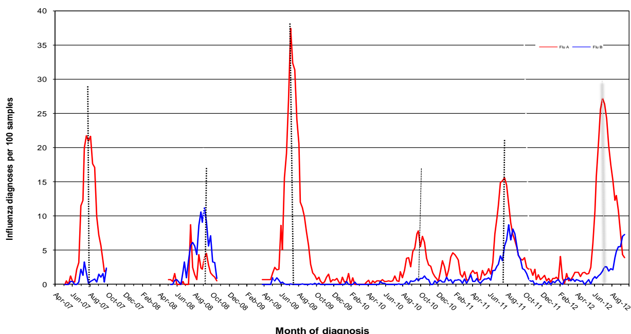
Figure 4: Percent of respiratory samples positive for influenza A or influenza B, 1 January 2007 – 21 September 2012, New South Wales.
