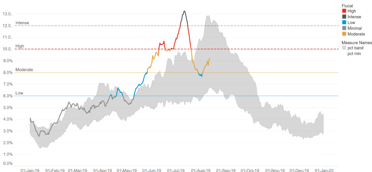
Figure 10: Healthdirect Australia – weekly ILI-related calls as a proportion of all calls for NSW, 2019 to the week ending 11 August compared to the weekly range between 2013 and 2018.
