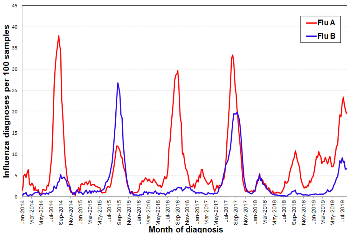
Figure 6: Percentage of laboratory tests positive for influenza A and influenza B by week, 1 January 2014 to 11 August 2019, New South Wales.
