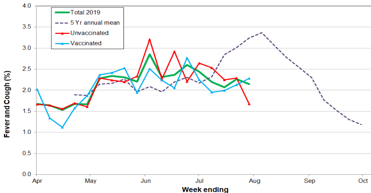
Figure 9: FluTracking – Percent of NSW participants reporting fever and cough by vaccination status and week, April to the week ending 11 August 2019, compared to the age standardised 5 year mean.
