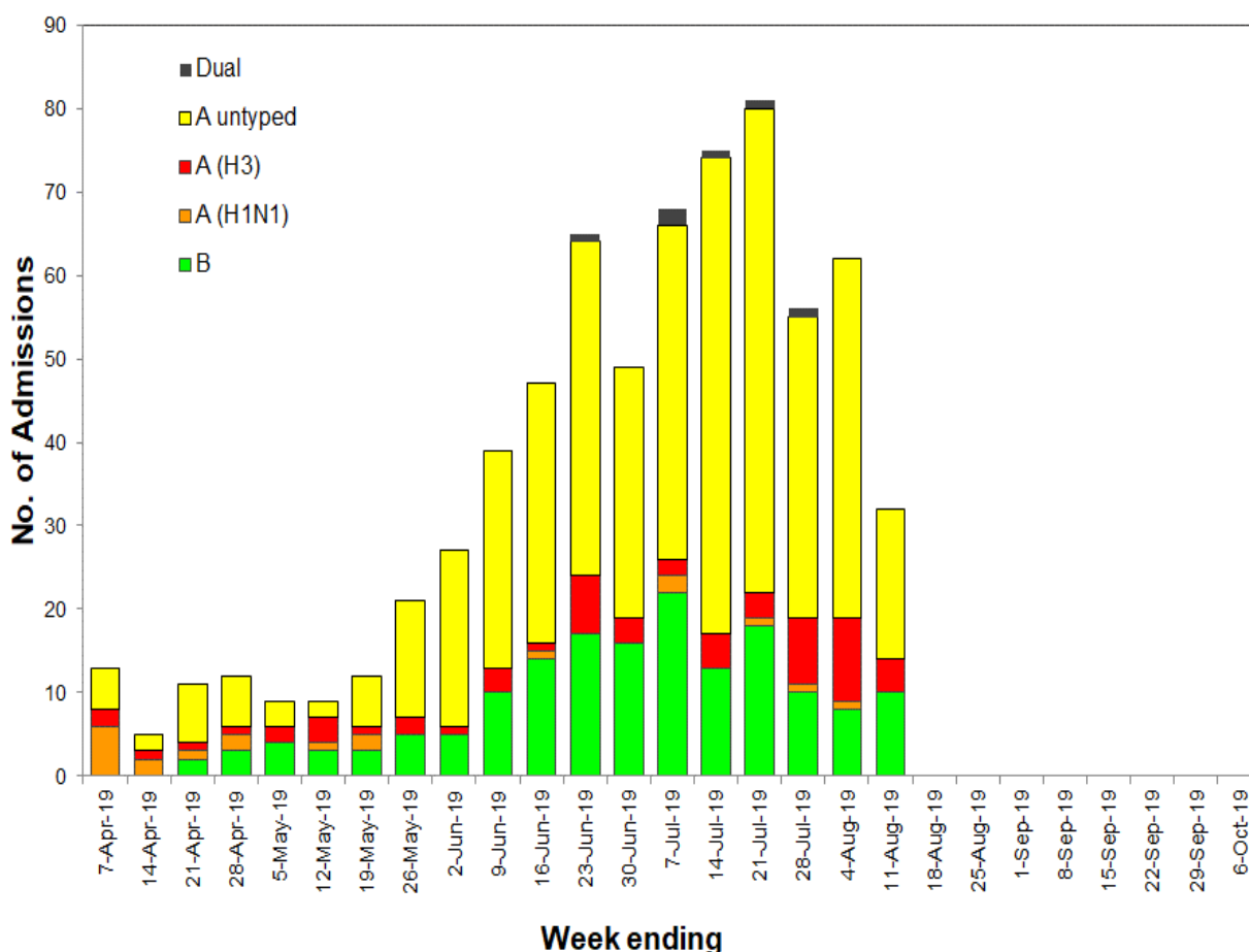
Figure 4: FluCAN – Confirmed influenza hospital admissions in NSW, 1 April – 11 August, 2019*.
