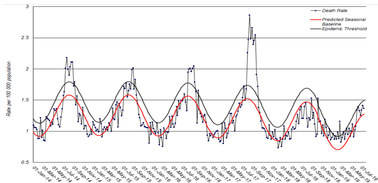
Figure 11: Rate of death registrations classified as influenza or pneumonia per 100,000 NSW population, 2014 – 19 July, 2019
