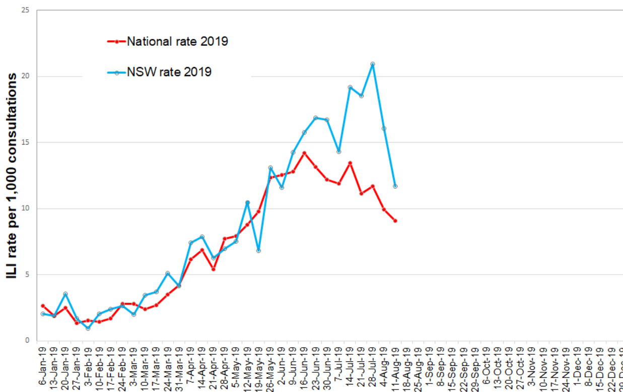
Figure 8: ASPREN – NSW and National GP ILI rates per 1000 consultations – 2019 to the week ending 11 August.
