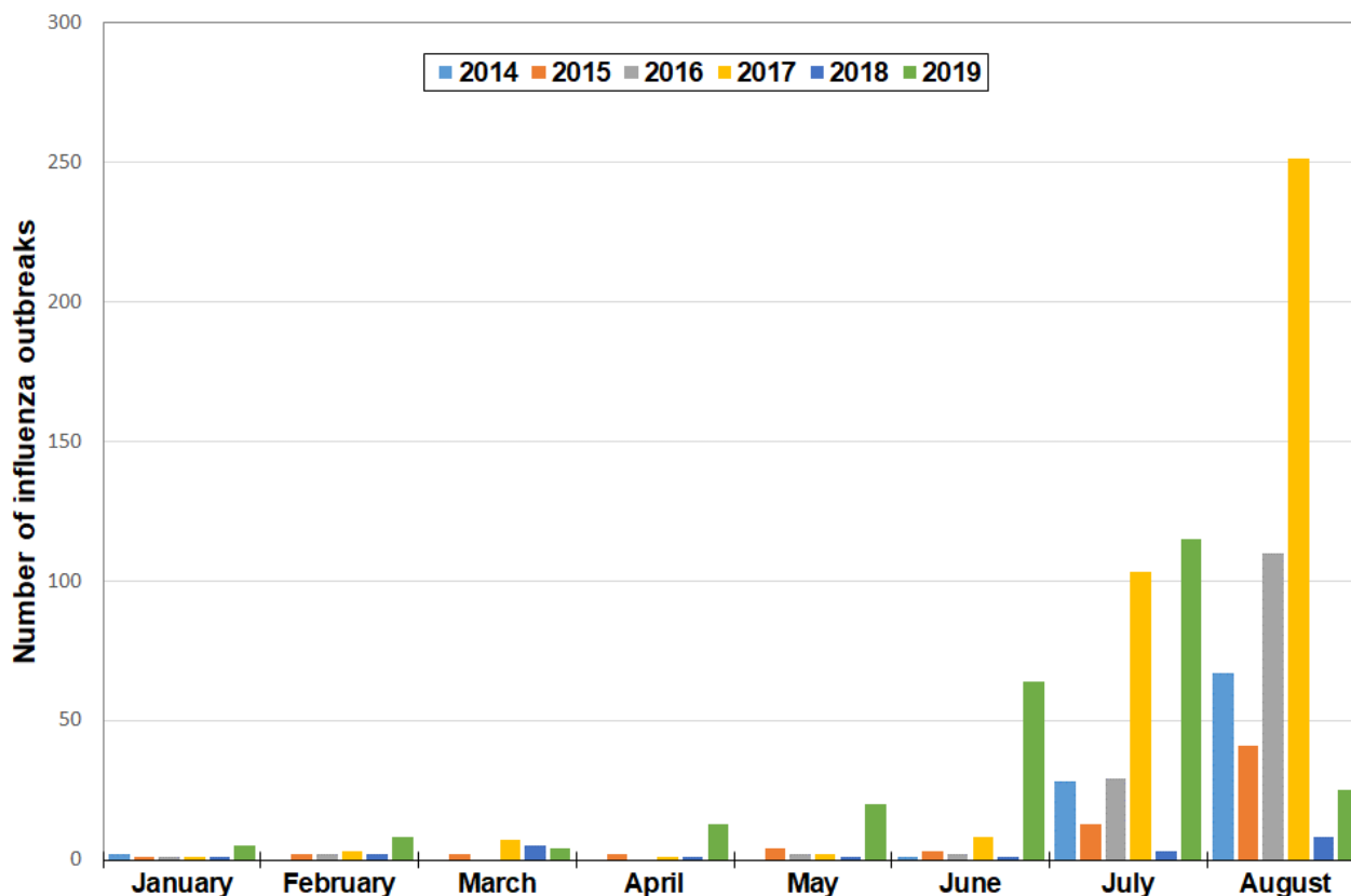
Figure 7: Reported influenza outbreaks in NSW residential care facilities by month, 2016 to 11 August 2019.
