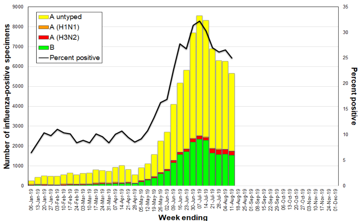
Figure 5: Weekly influenza positive test results by type and sub-type reported by NSW sentinel laboratories, 1 January to 11 August 2019.
