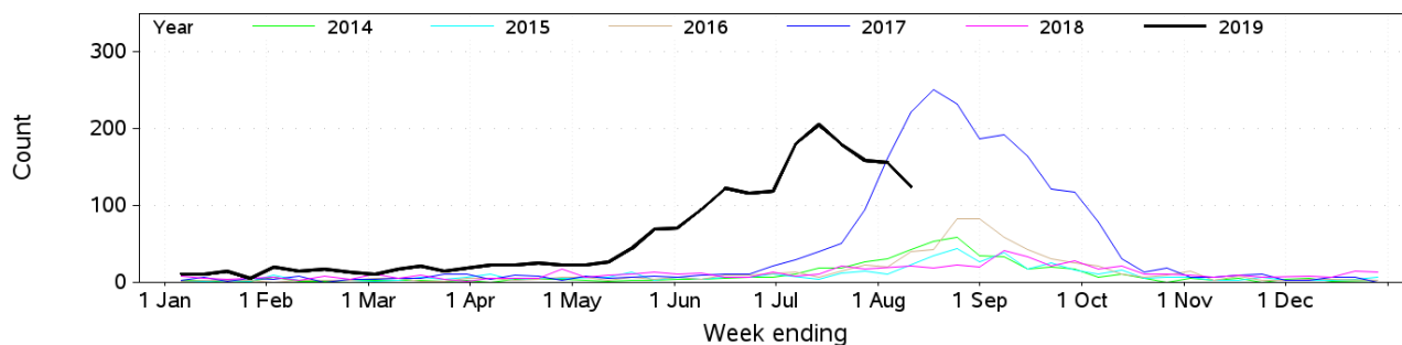
Figure 3: Total weekly counts of ED presentations for influenza-like illness or pneumonia, that were admitted to a critical care ward , all ages, 1 January – 11 August 2019 (black line), compared with the 5 previous years (coloured lines).
