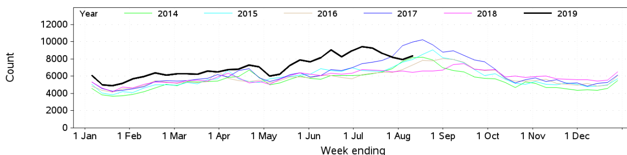
Figure 1: Total weekly counts of ED visits for All respiratory illness, fever and unspecified infections , all ages, 1 January – 11 August 2019 (black line), compared with the 5 previous years (coloured lines).
