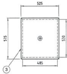
LID PLAN VIEW
