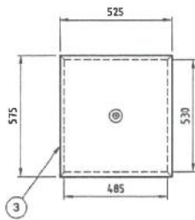
LID PLAN VIEW
