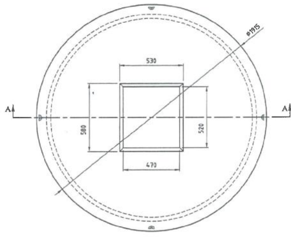
LID PLAN VIEW
