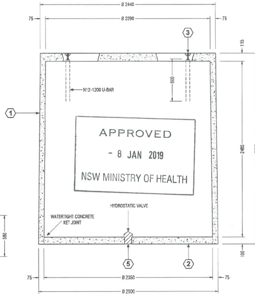
SECTION A-A (TANK)
