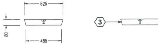
COVER DETAIL
